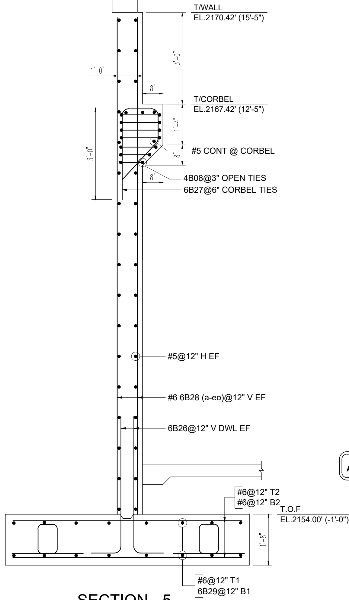
SECTION - 5 SCALE: 1/2" = 1'-0" REF: 1/GS2-1
