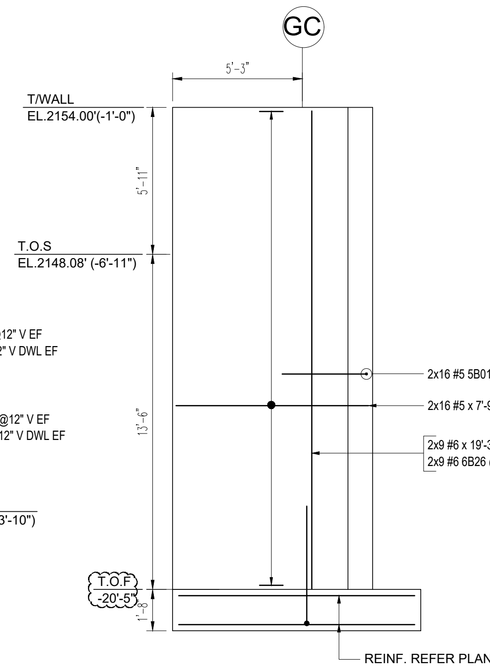
ELEVATION - N SCALE: 1/4" = 1'-0" REF: GS1-1
