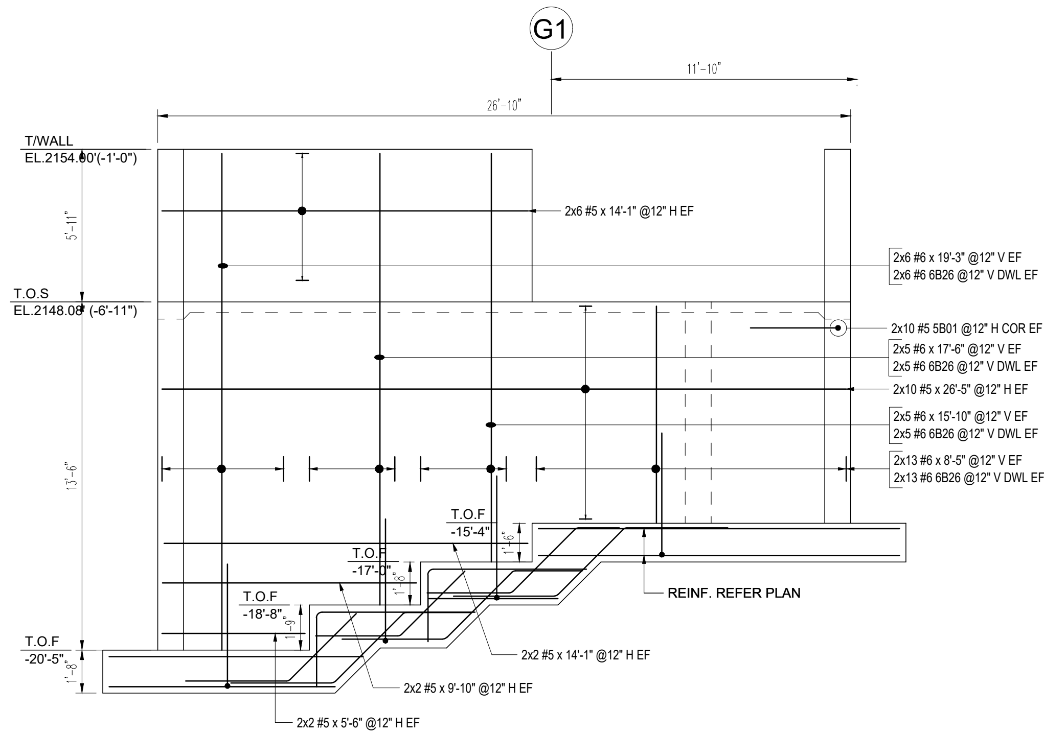
ELEVATION - K SCALE: 1/4" = 1'-0" REF: GS1-1
