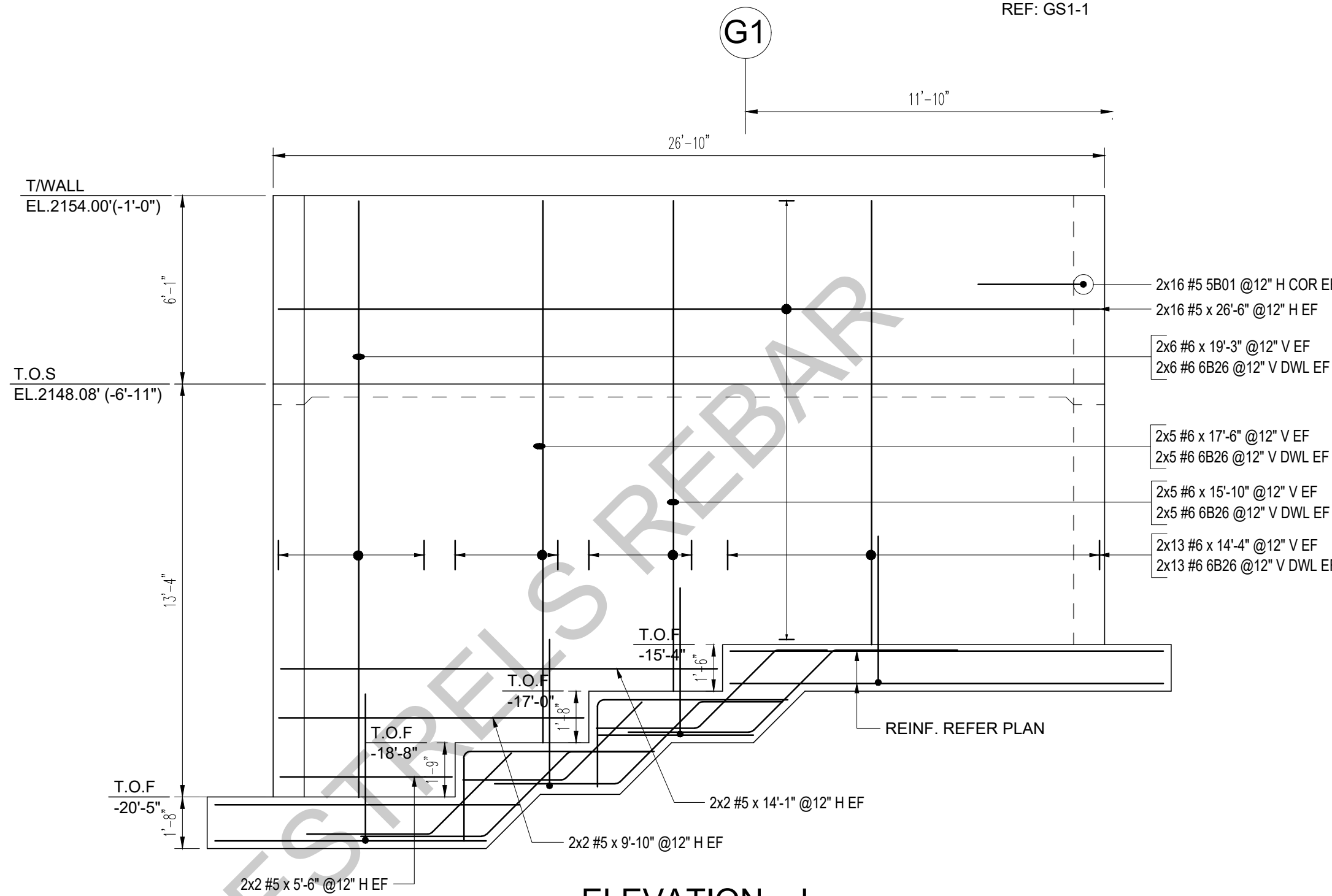
ELEVATION - J SCALE: 1/4" = 1'-0" REF: GS1-1
