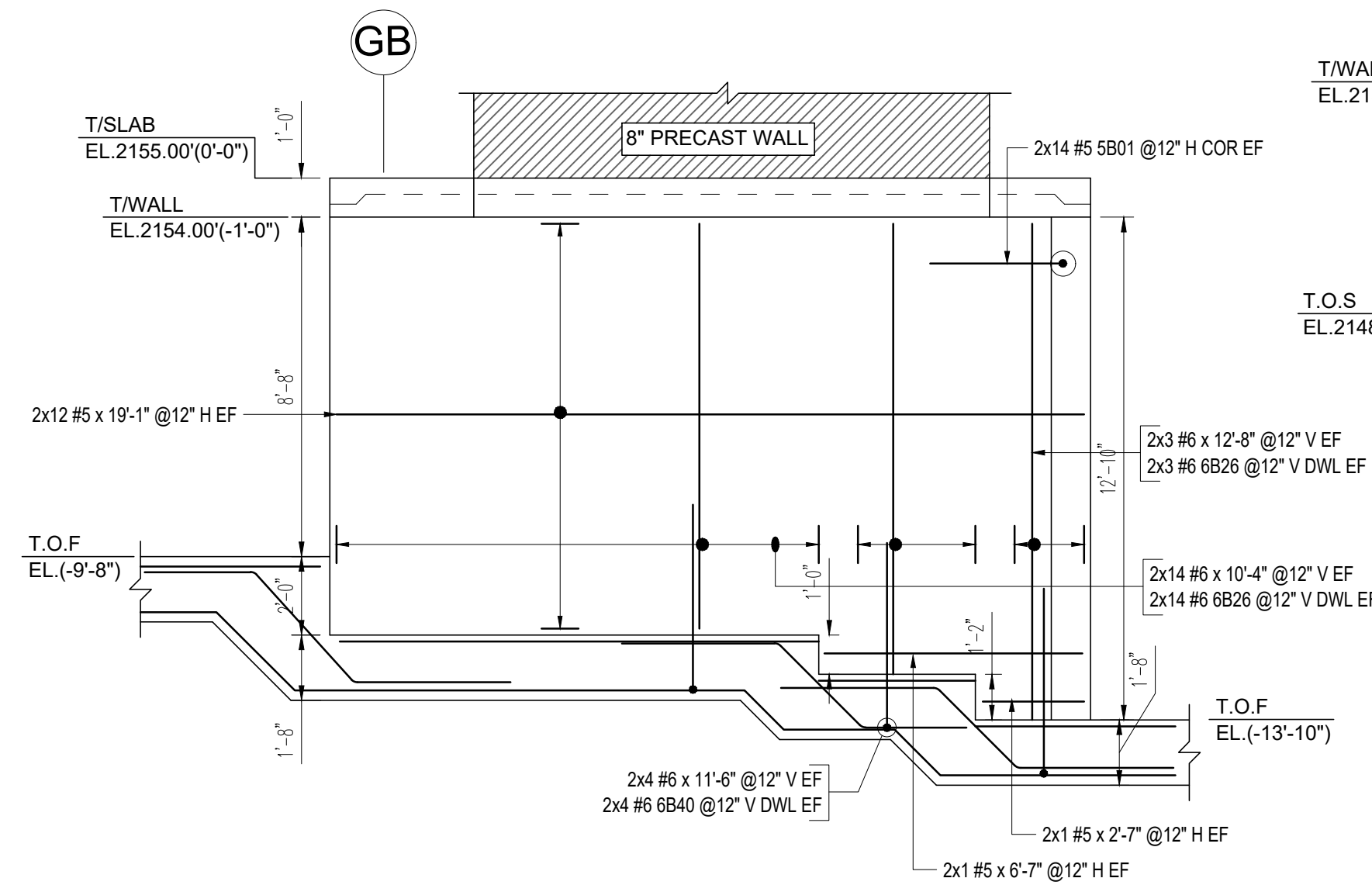
ELEVATION - M SCALE: 1/4" = 1'-0" REF: GS1-1
