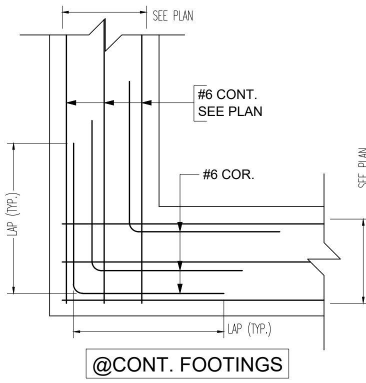
TYPICAL CORNER DETAIL SCALE: 1/2" = 1'-0"
