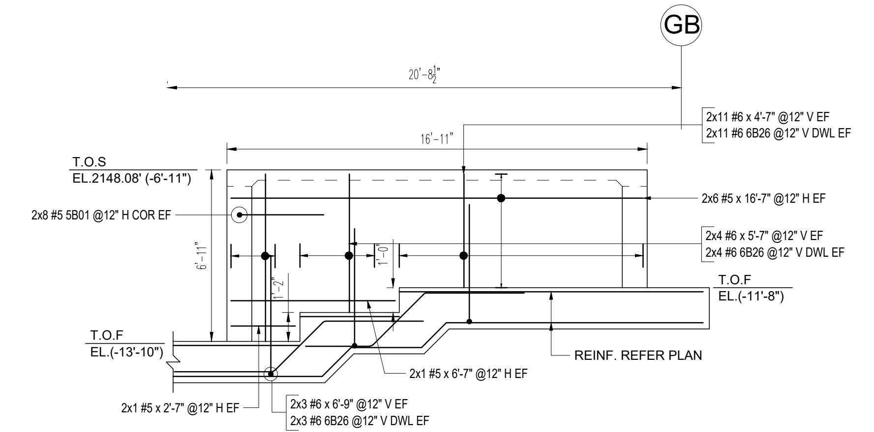
ELEVATION - L SCALE: 1/4" = 1'-0" REF: GS1-1
