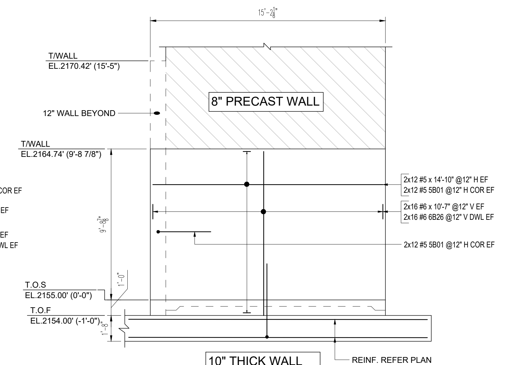
ELEVATION - O SCALE: 1/4" = 1'-0" REF: GS1-1
